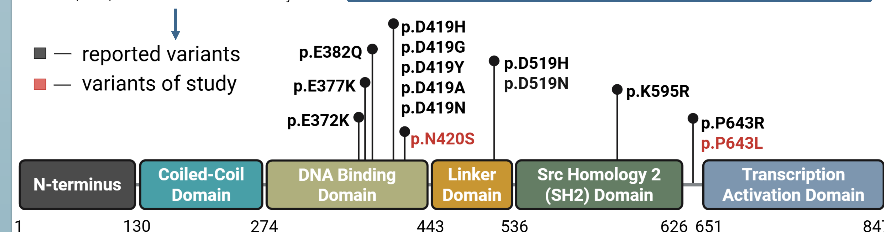
Fig.5: Schematic representation of STAT6 protein domain architecture mapping reported gain-of-function (GOF) variants and variants of study
